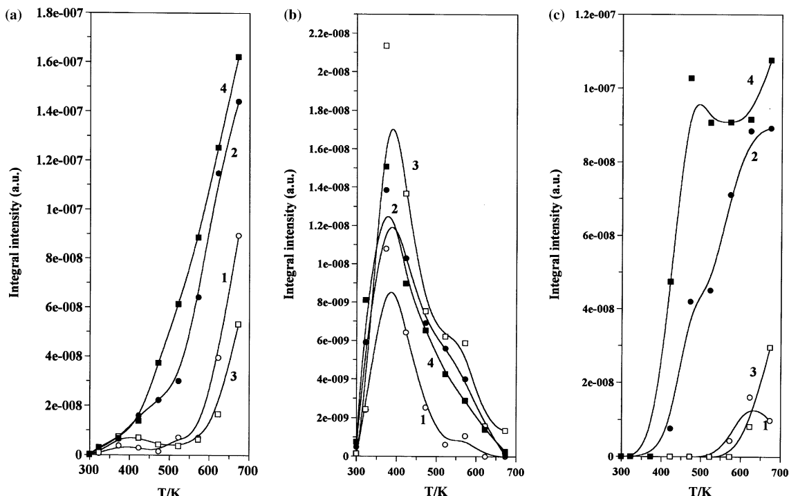
Figure 5. Formation of some gas phase products (monitored by MS) during the heat treatments (see text) of adsorbed acetaldehyde layer on reduced catalysts: 1 – \text{Al}_2\text{O}_3 ; 2 – 1% \text{Rh}/\text{Al}_2\text{O}_3 ; 3 – 1% \text{Au}/\text{Al}_2\text{O}_3 and 4 – 1% \text{Pt}/\text{Al}_2\text{O}_3 . (a) hydrogen; (b) ethane and (c) ethylene.
